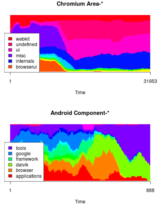
Figure 1: SUBCOMPONENT class distribution change over time
