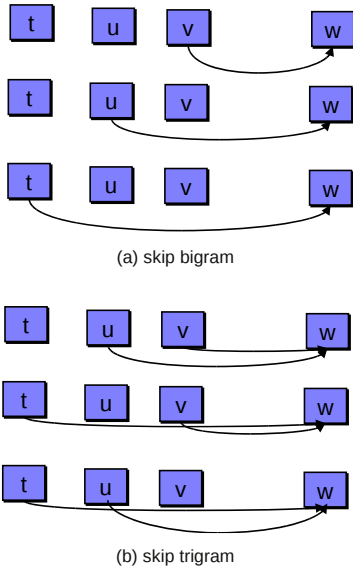
Figure 1: The skip bigram and the skip trigram models over a window of four words
