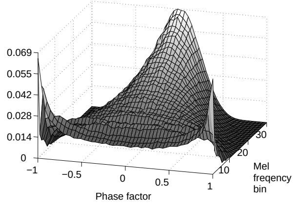
Figure 2: Empirical distribution of the phase factors \alpha_i .
