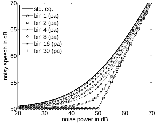
Figure 1: Noisy speech power y as a function of noise power n in the log-Mel domain calculated with the standard model (3), as well as with the phase-averaged model (8) proposed in this paper. Note that the averages are dependent on the frequency bin.
