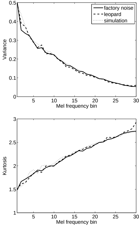
Figure 3: Variance and kurtosis of the distribution of phase factors for the simulation, tank (leopard) and factory noise
