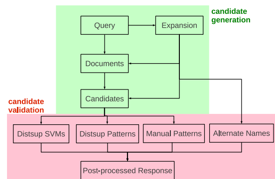
Figure 2: Data flow of the relation extraction system: The candidate generation stage retrieves possible relational contexts. The candidate validation stage predicts whether relations actually hold and produces a valid response.
