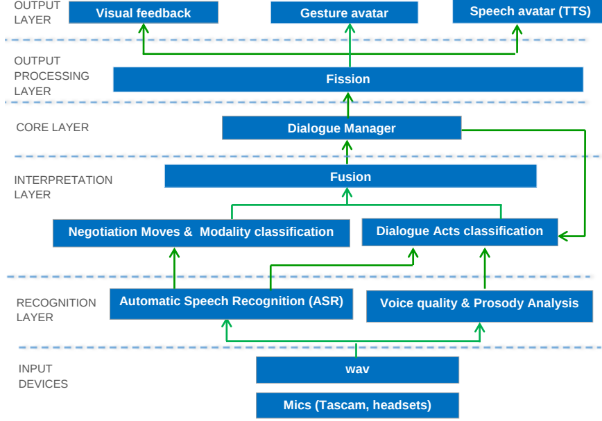
Figure 2: Architecture of the Virtual Negotiation Coach system.
