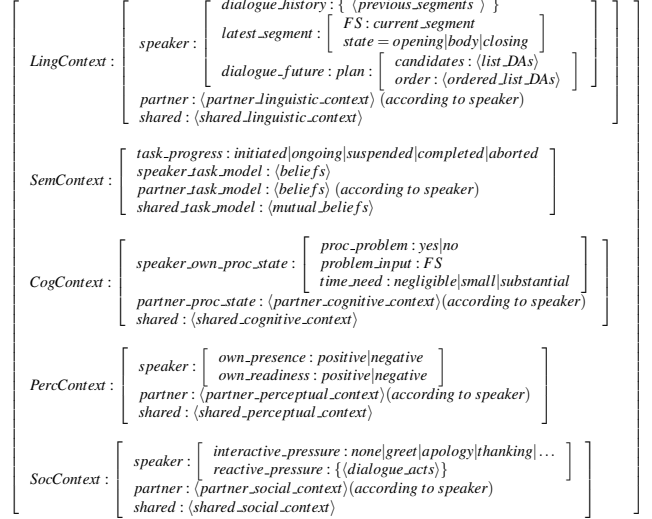
Figure 4: Feature structure representation of the context model.
